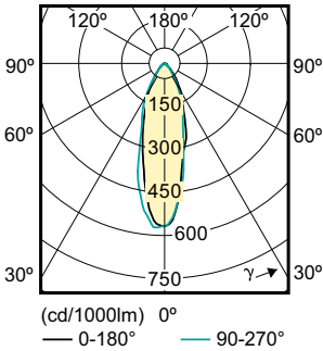
Light Distribution Diagram - Corepro LEDspot 3.5-35W GU10 827 36D
